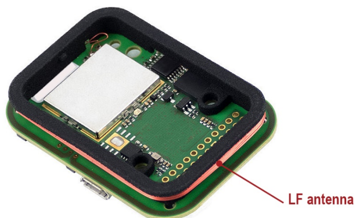
TWN4 MultiTech 3 M LF – bottom view
