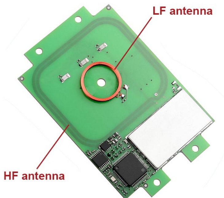
PCB contained in TWN4 MultiTech 2 LEGIC LF HF (exemplary picture)
