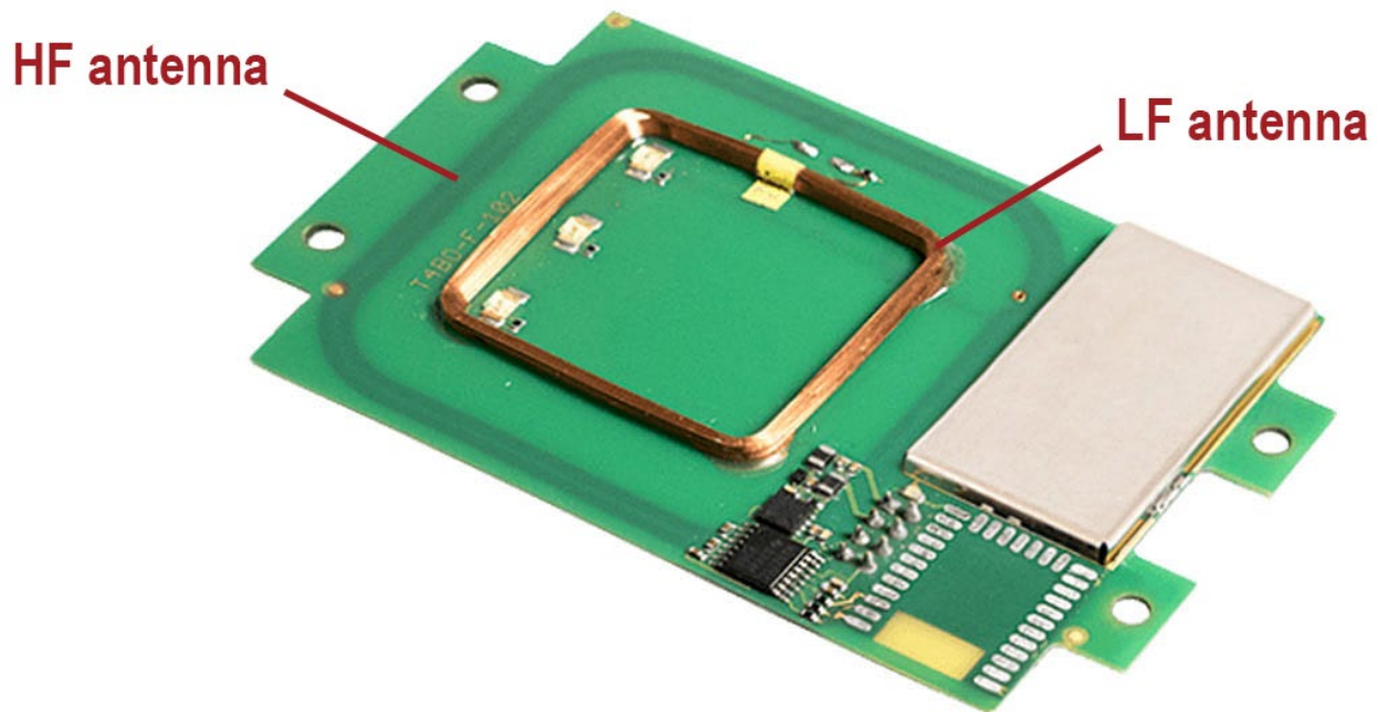
PCB contained in TWN4 MultiTech 2 LF HF
