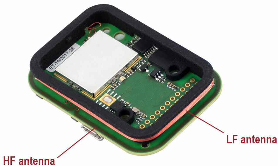
TWN4 MultiTech 3 LEGIC M LF HF
