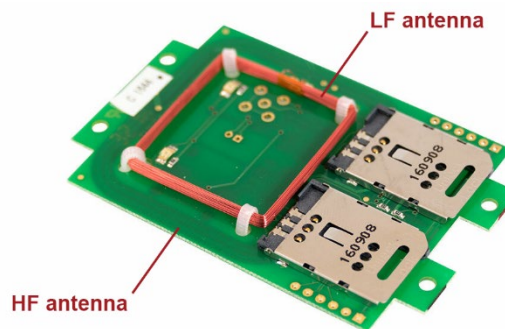
TWN4 MultiTech LEGIC M
