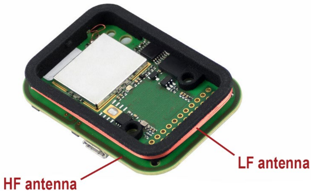
PCB contained in TWN4 USB Front Reader
